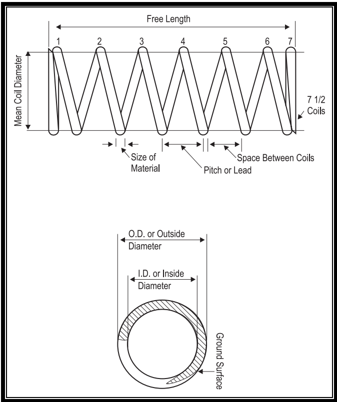
Figure ST-3. Dimensional Terminology for Helical Compression Springs.
